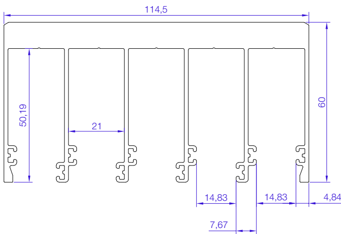
MARCO SUPERIOR 5 CARRILES
